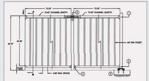
Guardrail Details
