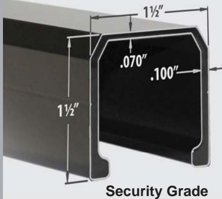
Security Picket
