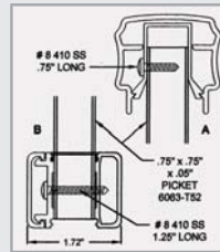
Intermediate Bracket
